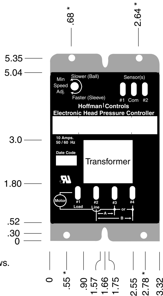
812/814/816 -10E Series Control Dimensions
