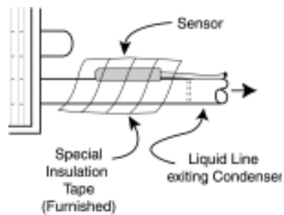
Figure 1 - Sensor Installation
