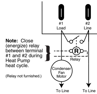
Figure 3 Wiring Modifications for Heat Pump Applications 812/814/816 -10D and -10E
