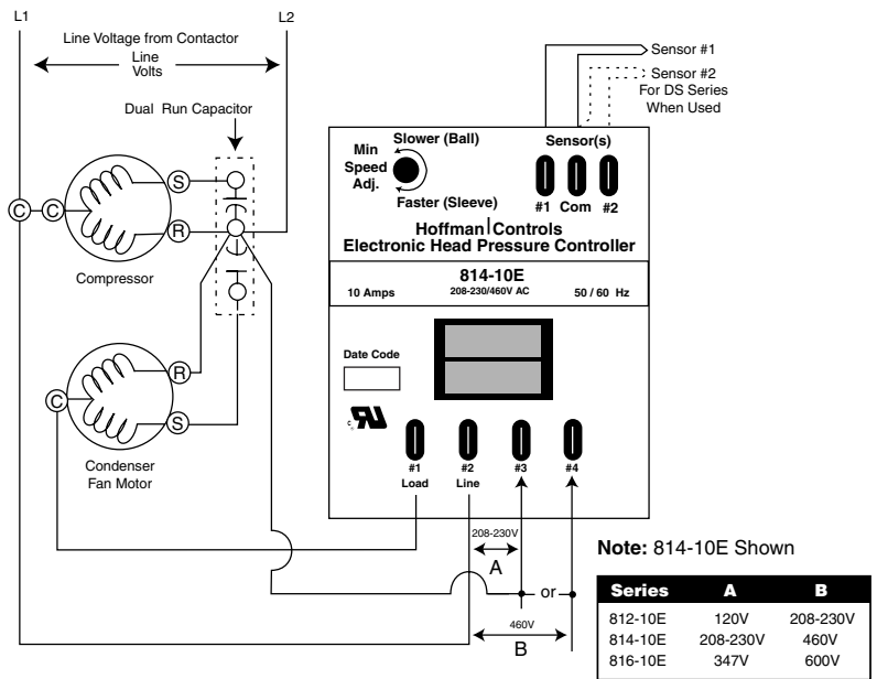
Figure 1c Dual Run Capacitor Wiring Diagram for the -10E Series
