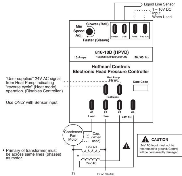
Figure 1d Wiring Diagram for the 816-10D (HPVD)
