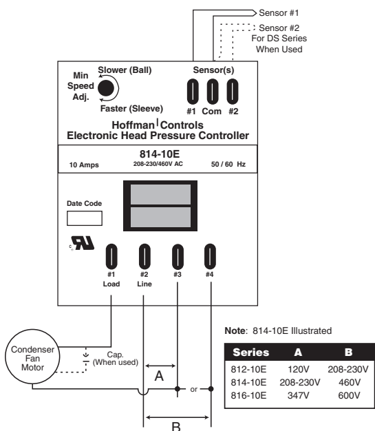
Figure 1a Wiring for 814-10E and 814-10EDS
