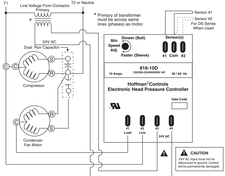
Figure 1b Dual Run Capacitor Wiring Diagram for the -10D Series
