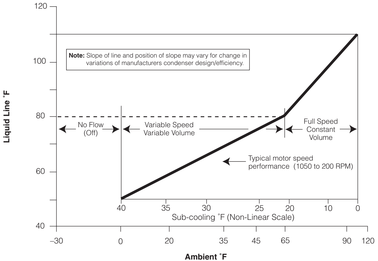
Figure 4 Liquid °F vs. Ambient °F and Sub-cooling °F
