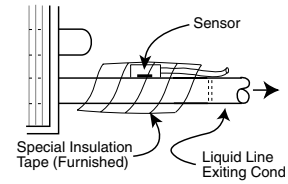
Figure 2 Sensor Mounting
